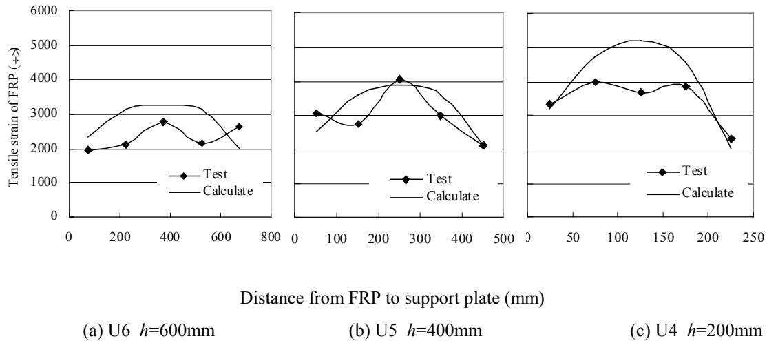
Figure 8 Measured FRP strain distribution along the diagonal crack versus FE prediction
